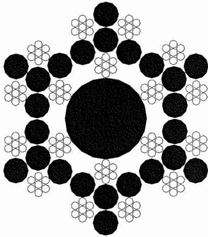
FIGURE 32. Type III, marine (cables), class 4, 6 by 3 by 7 spring lay.
