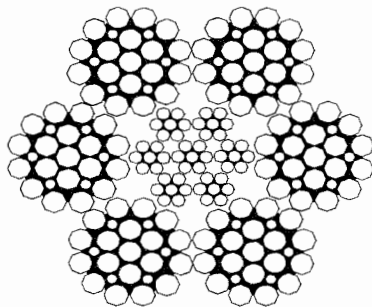
FIGURE 3. Independent wire-rope core (IWRC).
