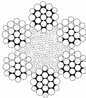
FIGURE 7. Type I, general purpose, class 2, construction 2, 6 by 19 (Warrington), and type II, elevator, class 1, construction 1, 6 by 19 (Warrington).
