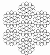
FIGURE 52. Type VI, small cords, class 3 7 by 19 (2 operations).
