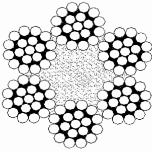
FIGURE 1. Fiber core.
