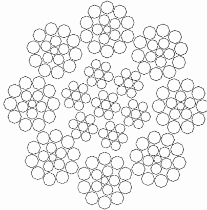
FIGURE 46. Type IV, miscellaneous, class 4, construction 2, 8 by 19 rotation resistant (Filler wire).
