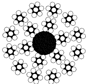
FIGURE 40. Type IV, miscellaneous, class 2, 18 by 7 rotation resistant.
