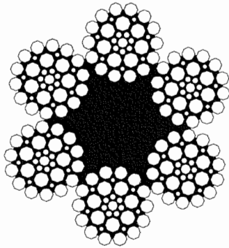
FIGURE 17. Type I, general purpose, class 3, construction 7, 6 by 36 (Seale-Filler wire).
