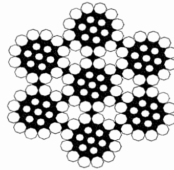
FIGURE 2. Wire strand core.
